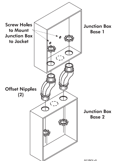
Junction box assembly dual base boilers
